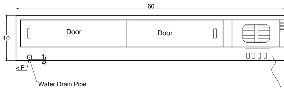
Rear view
