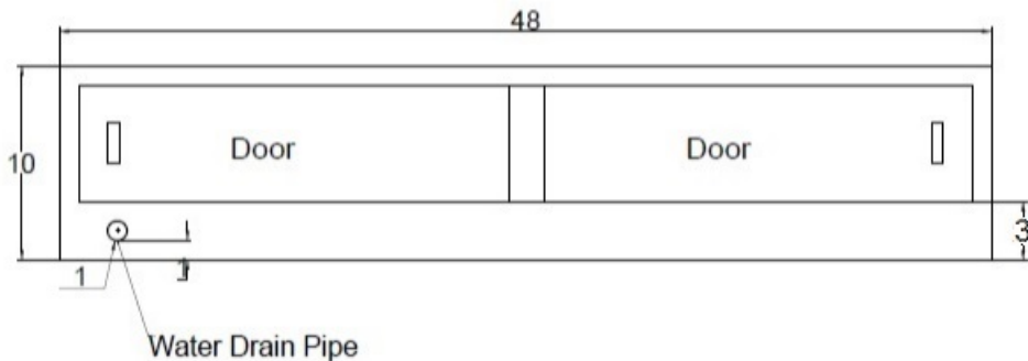
Rear view
