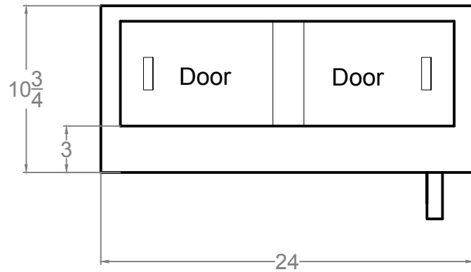
Rear view
